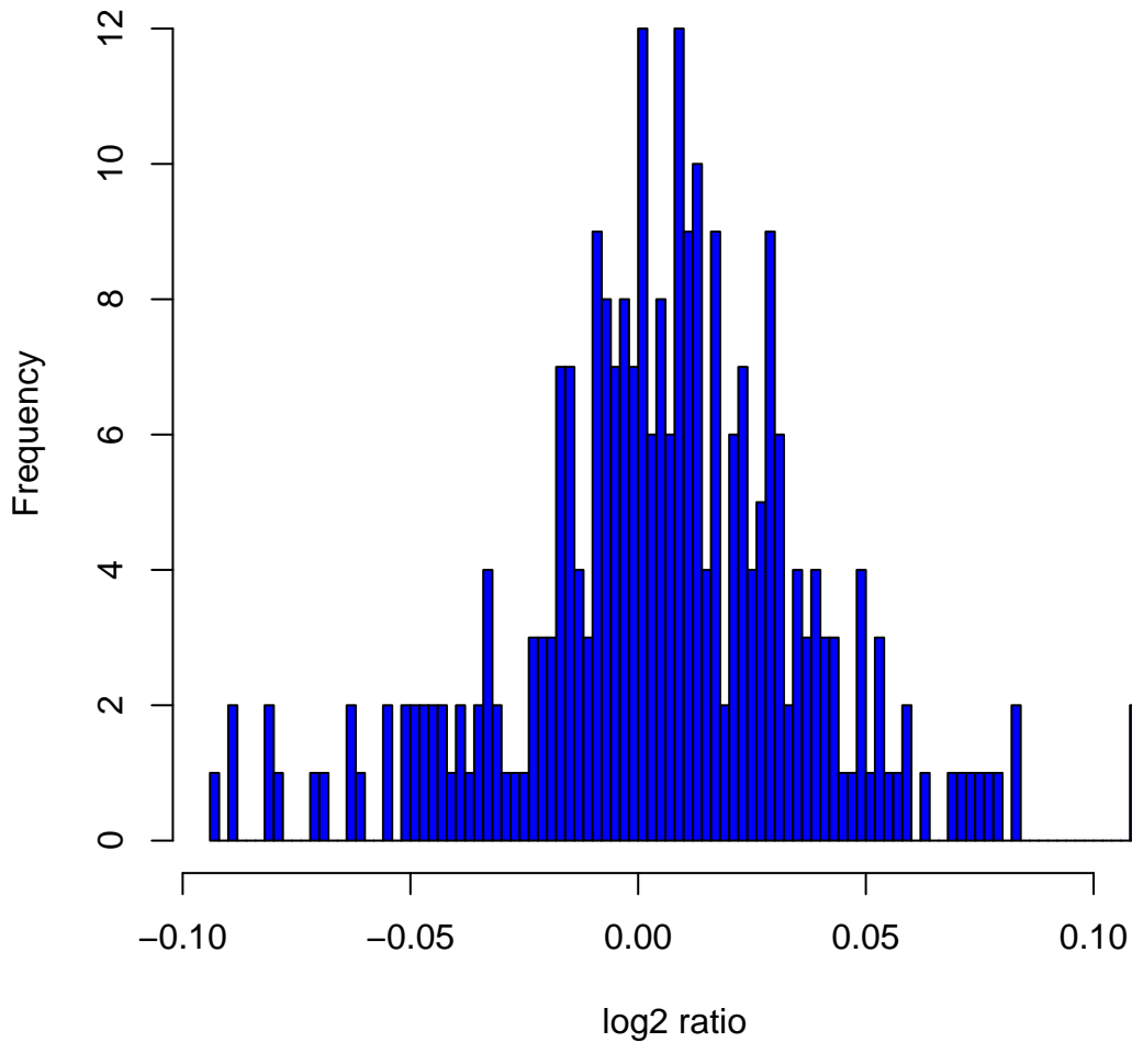
Histogram of log 2 ratios in 270 HapMap samples at clone Chr5tp-5B3
