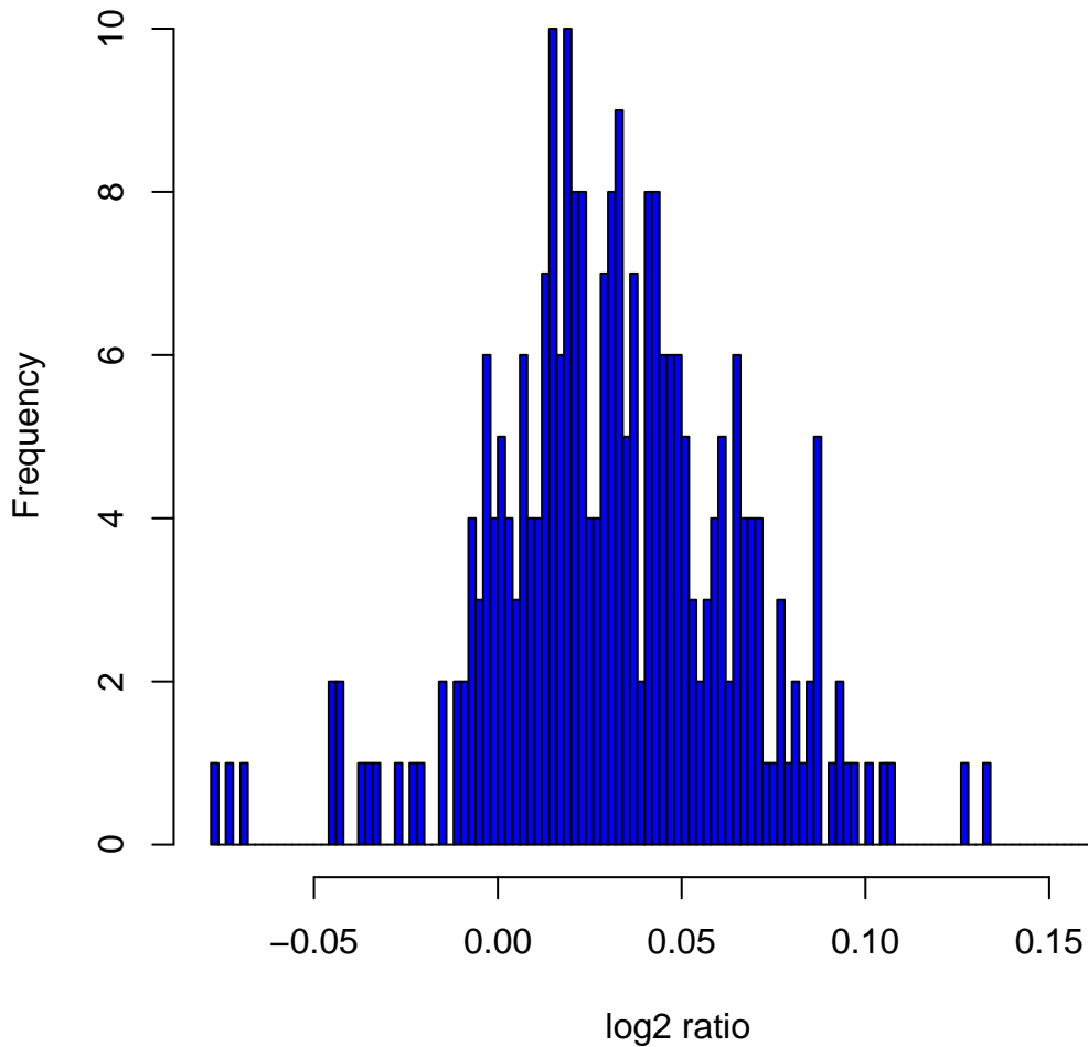
Histogram of log 2 ratios in 270 HapMap samples at clone Chr5tp-5B6
