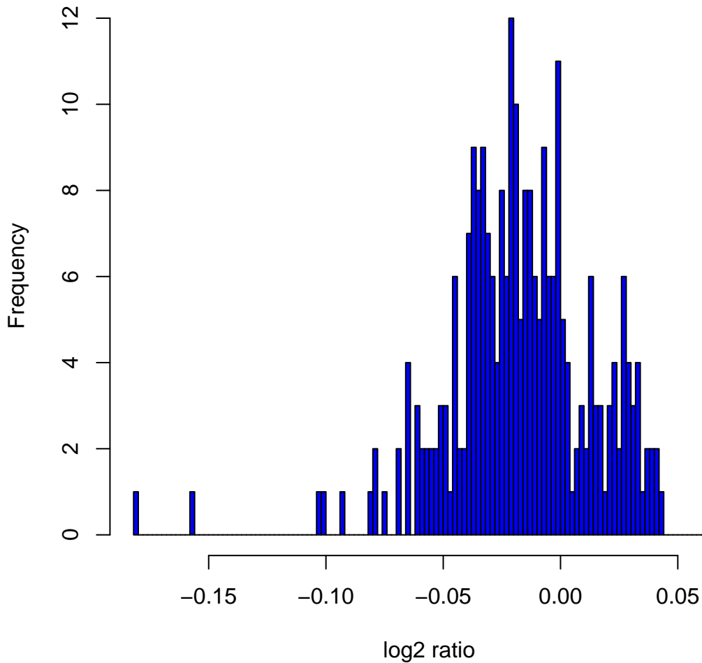
Histogram of log 2 ratios in 270 HapMap samples at clone Chr5tp-5B8
