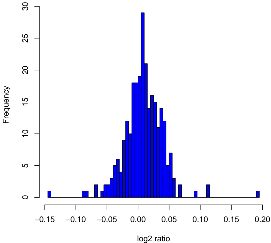
Histogram of \log_2 ratios in 270 HapMap samples at clone Chr5tp-5C4
