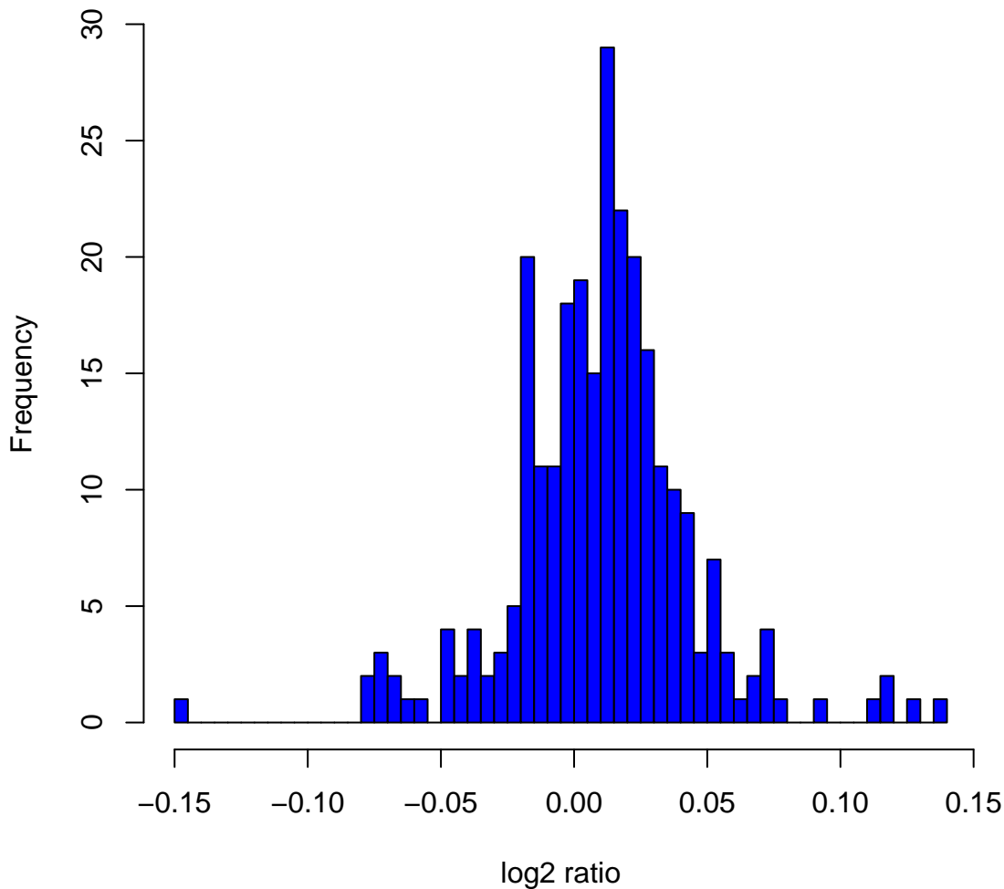
Histogram of log 2 ratios in 270 HapMap samples at clone Chr5tp-5C9
