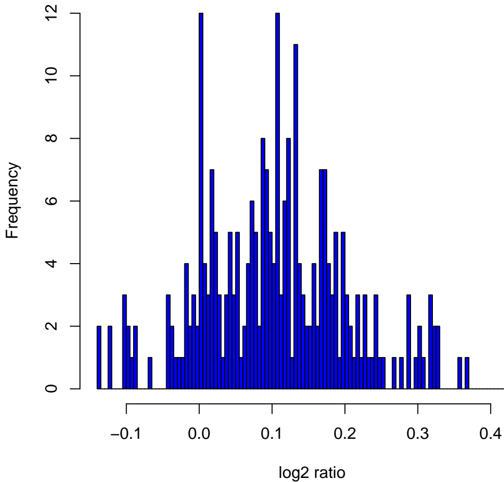
Histogram of log 2 ratios in 270 HapMap samples at clone Chr5tp-5D1
