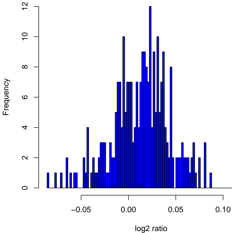
Histogram of log 2 ratios in 270 HapMap samples at clone Chr5tp-5D4
