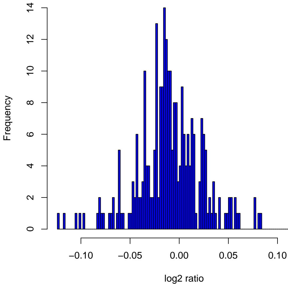
Histogram of \log_2 ratios in 270 HapMap samples at clone Chr5tp-5E11
