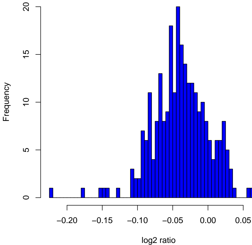
Histogram of log 2 ratios in 270 HapMap samples at clone Chr5tp-6A1
