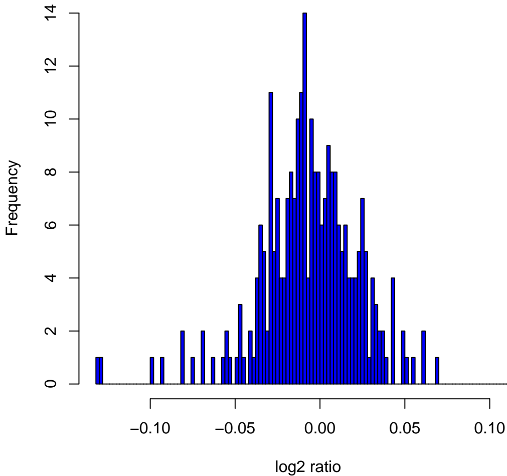
Histogram of \log_2 ratios in 270 HapMap samples at clone Chr5tp-6A5
