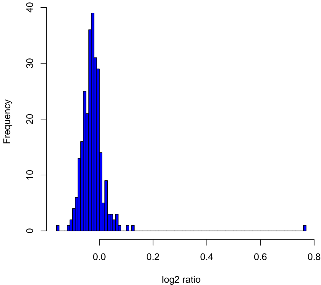
Histogram of log2ratios in 270 HapMap samples at clone Chr5tp-6B10
