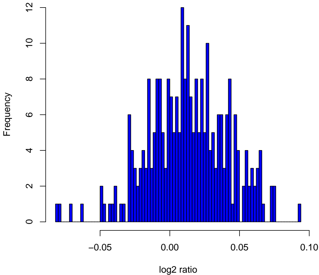
Histogram of log 2 ratios in 270 HapMap samples at clone Chr5tp-6C2
