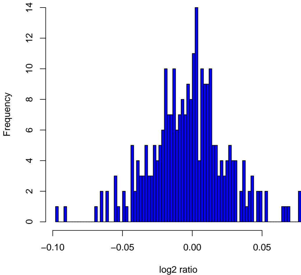
Histogram of log 2 ratios in 270 HapMap samples at clone Chr5tp-6C4
