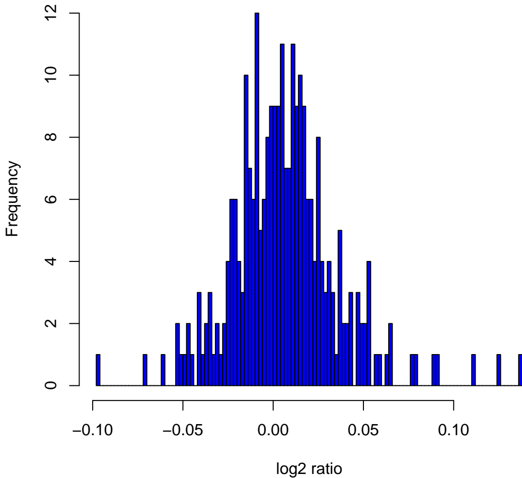
Histogram of \log_2 ratios in 270 HapMap samples at clone Chr5tp-6C8
