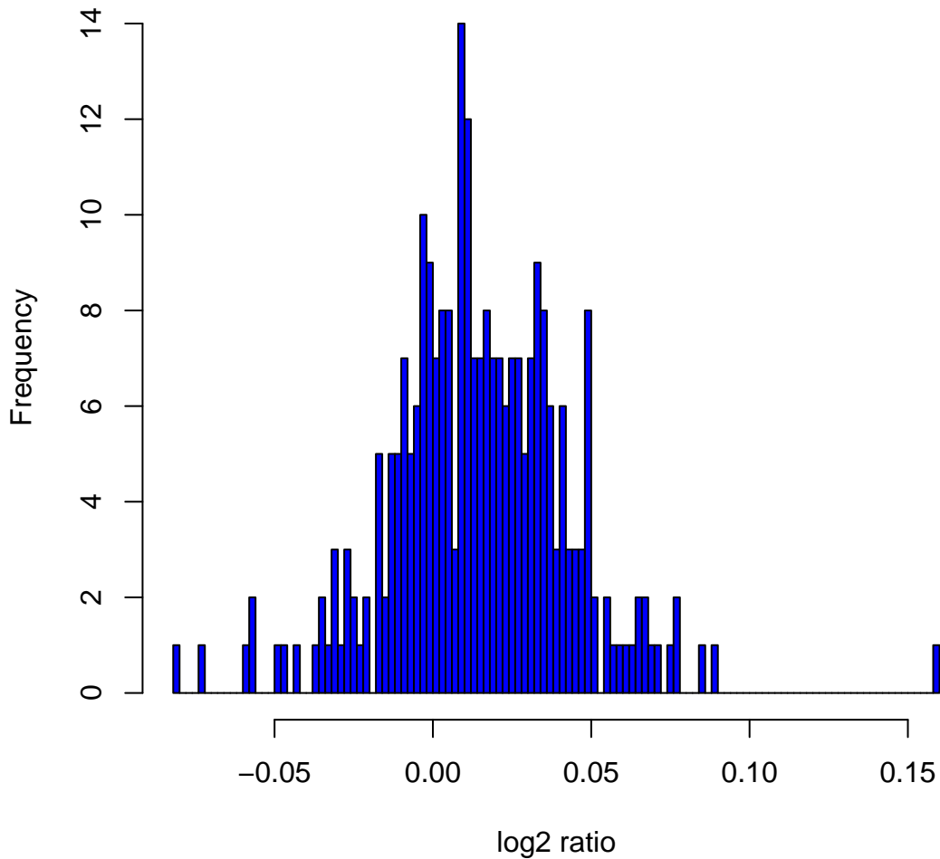
Histogram of \log_2 ratios in 270 HapMap samples at clone Chr5tp-6C9
