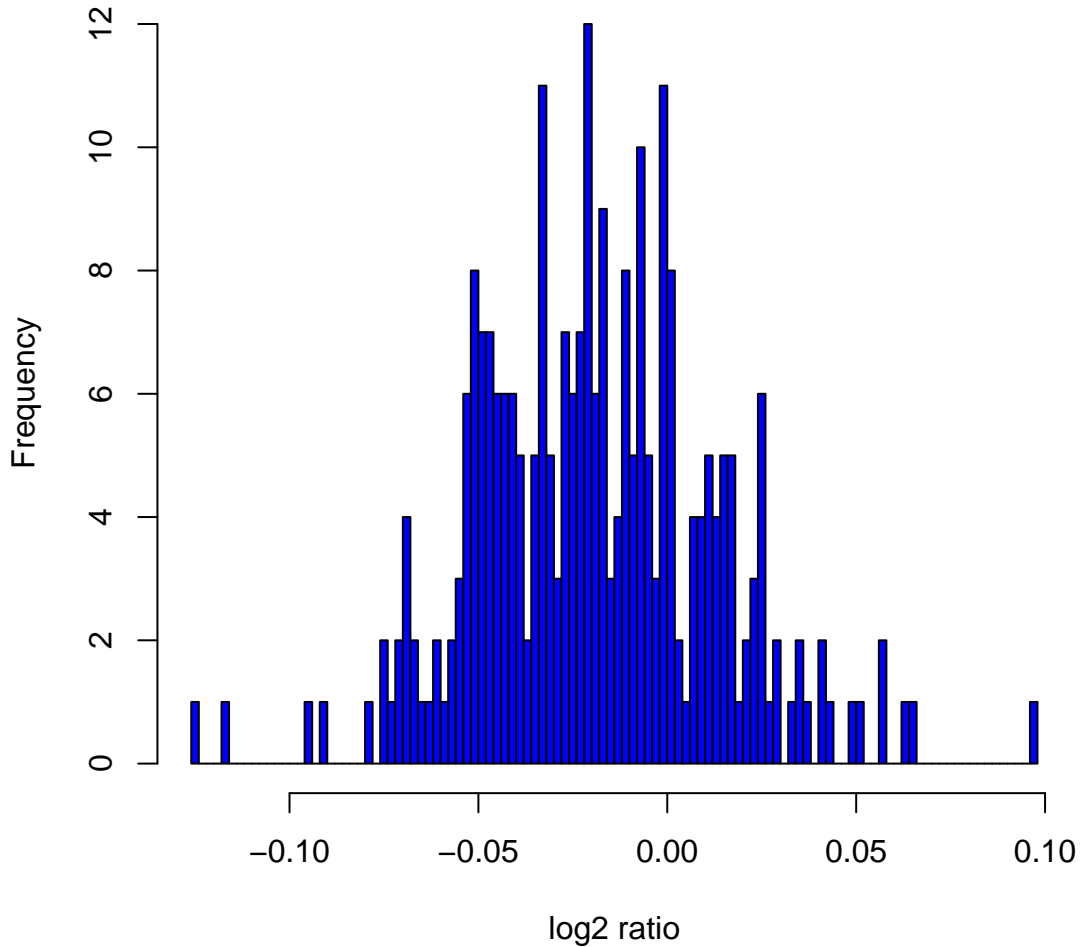
Histogram of log2ratios in 270 HapMap samples at clone Chr5tp-6F5
