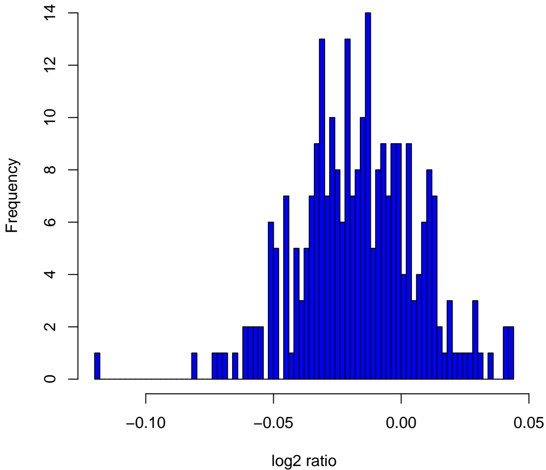
Histogram of log2ratios in 270 HapMap samples at clone Chr5tp-6F8
