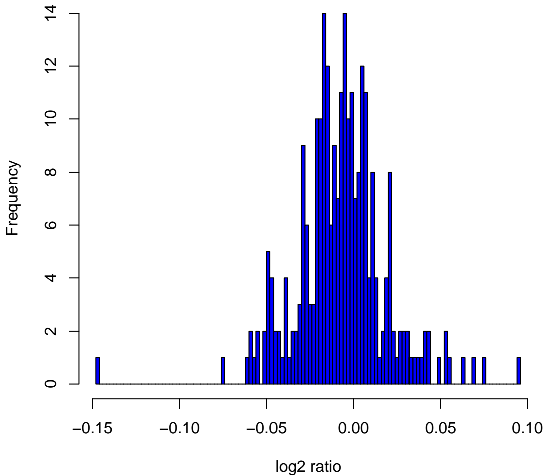
Histogram of \log_2 ratios in 270 HapMap samples at clone Chr5tp-6G7
