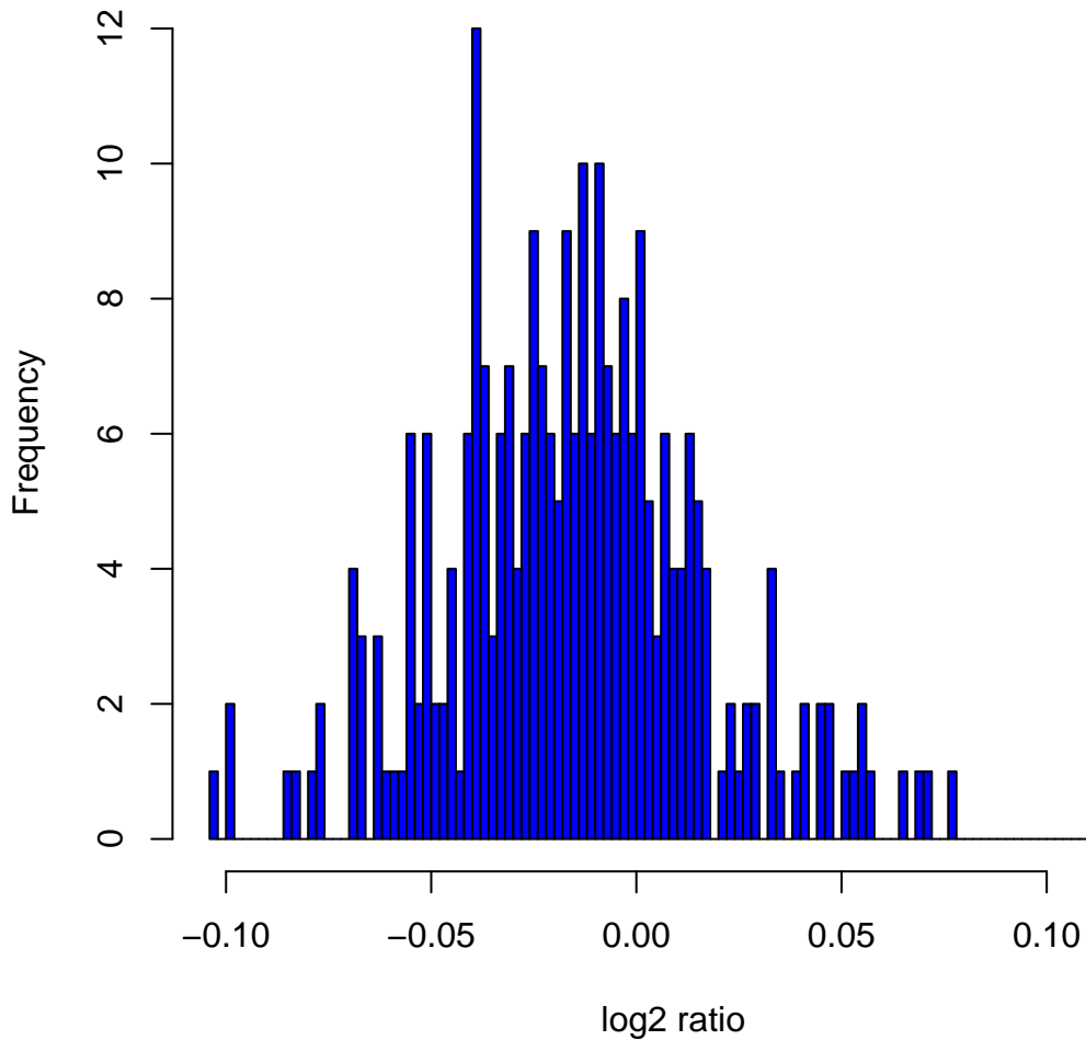
Histogram of log 2 ratios in 270 HapMap samples at clone Chr5tp-6H9
