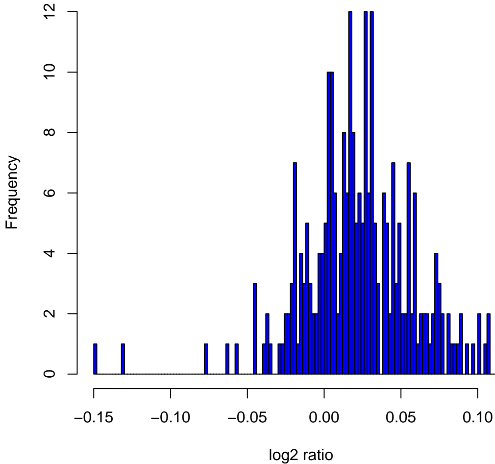
Histogram of log 2 ratios in 270 HapMap samples at clone Chr5tp-8A10
