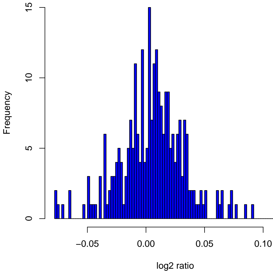
Histogram of log 2 ratios in 270 HapMap samples at clone Chr5tp-8A5
