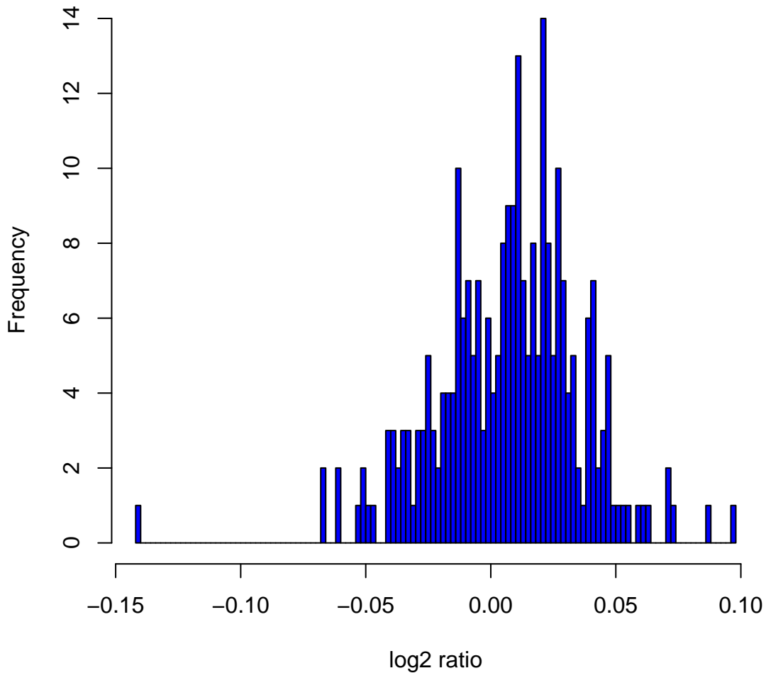
Histogram of log 2 ratios in 270 HapMap samples at clone Chr5tp-8A6
