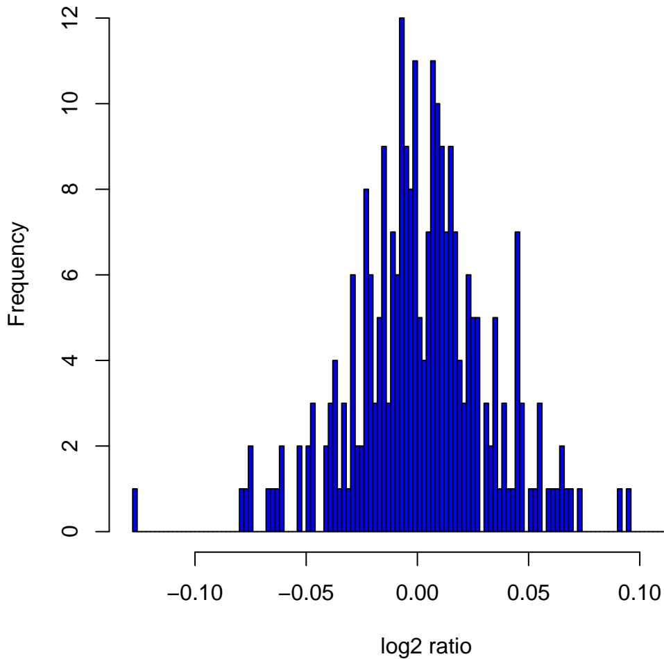
Histogram of \log_2 ratios in 270 HapMap samples at clone Chr5tp-8B6
