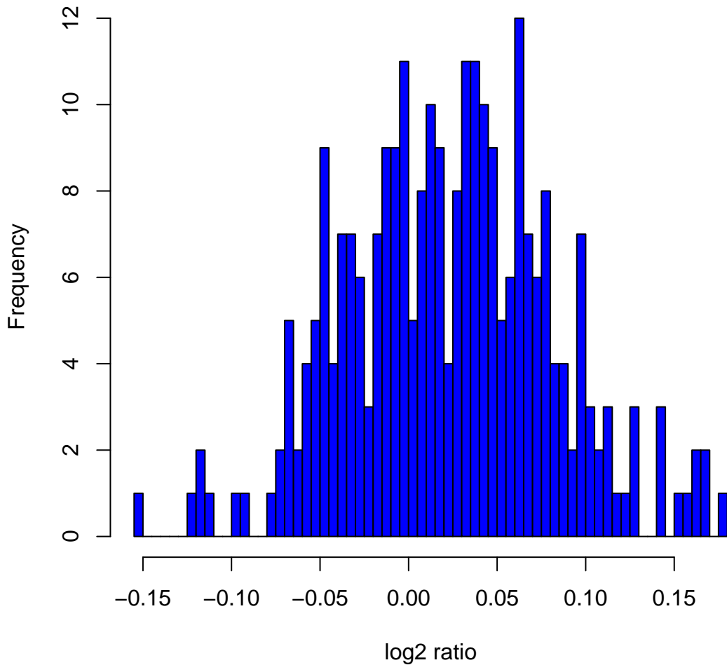
Histogram of log 2 ratios in 270 HapMap samples at clone Chr5tp-9A4
