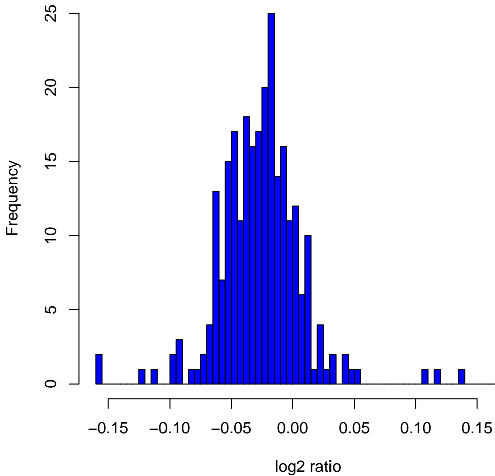
Histogram of \log_2 ratios in 270 HapMap samples at clone Chr5tp-9A7
