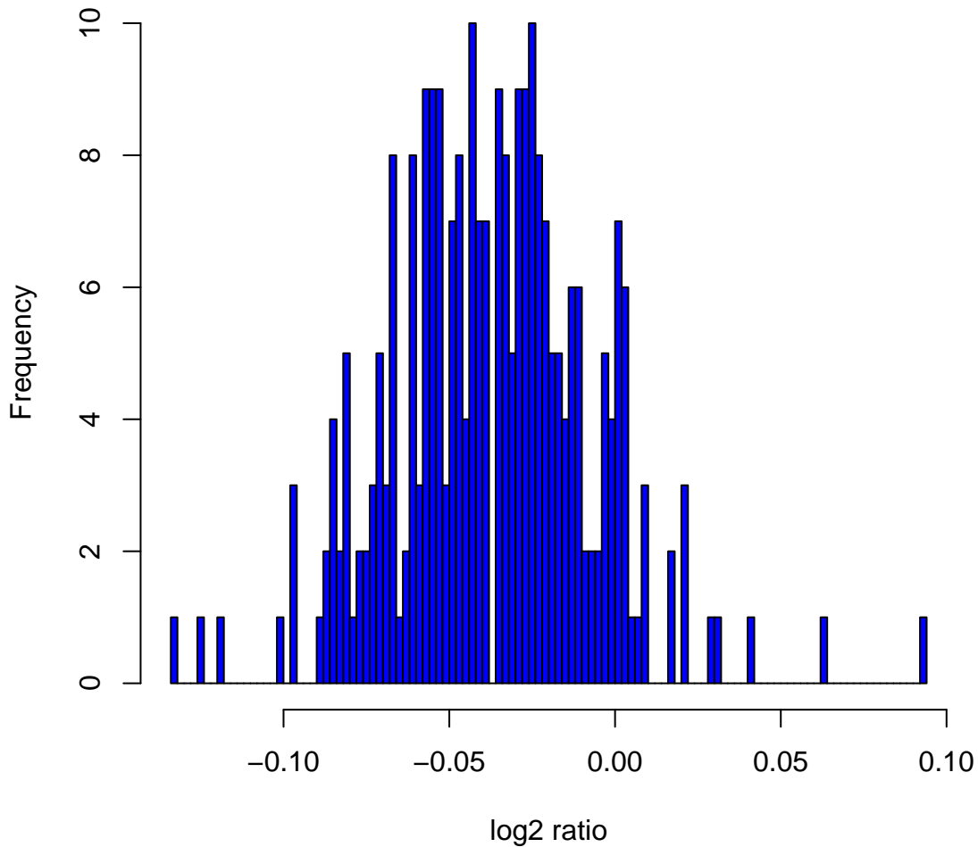
Histogram of \log_2 ratios in 270 HapMap samples at clone Chr5tp-9B5
