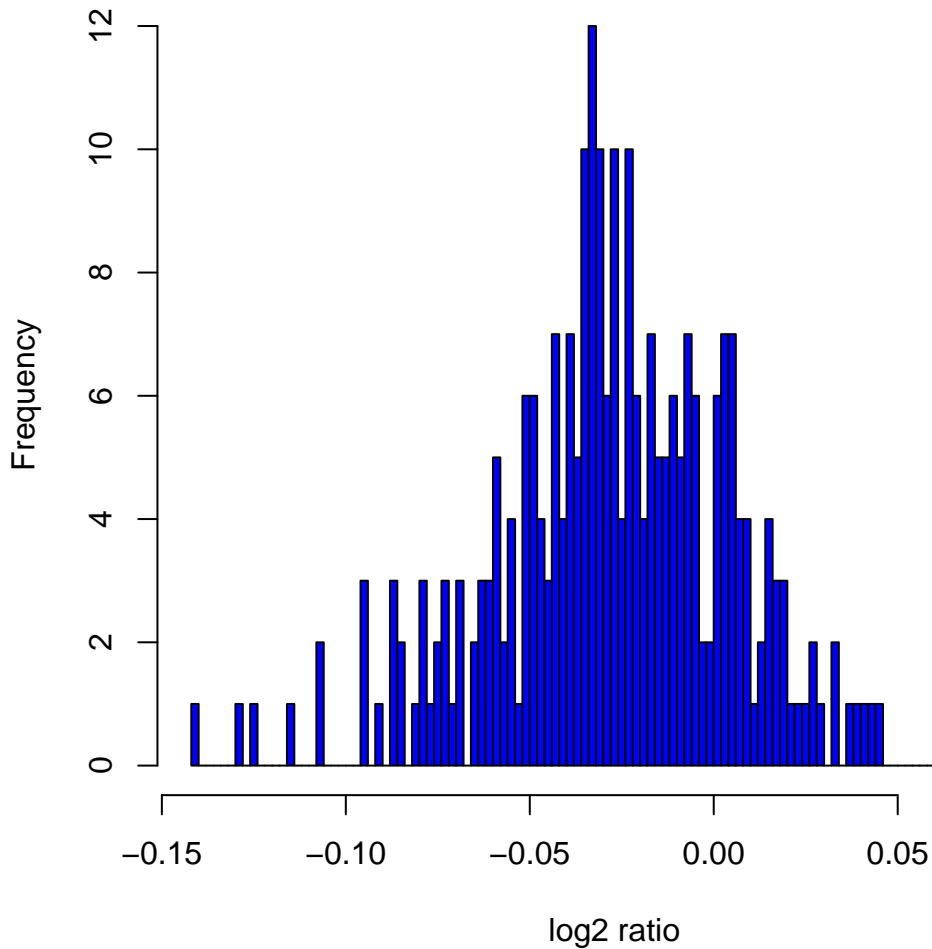
Histogram of log2ratios in 270 HapMap samples at clone Chr5tp-9D10
