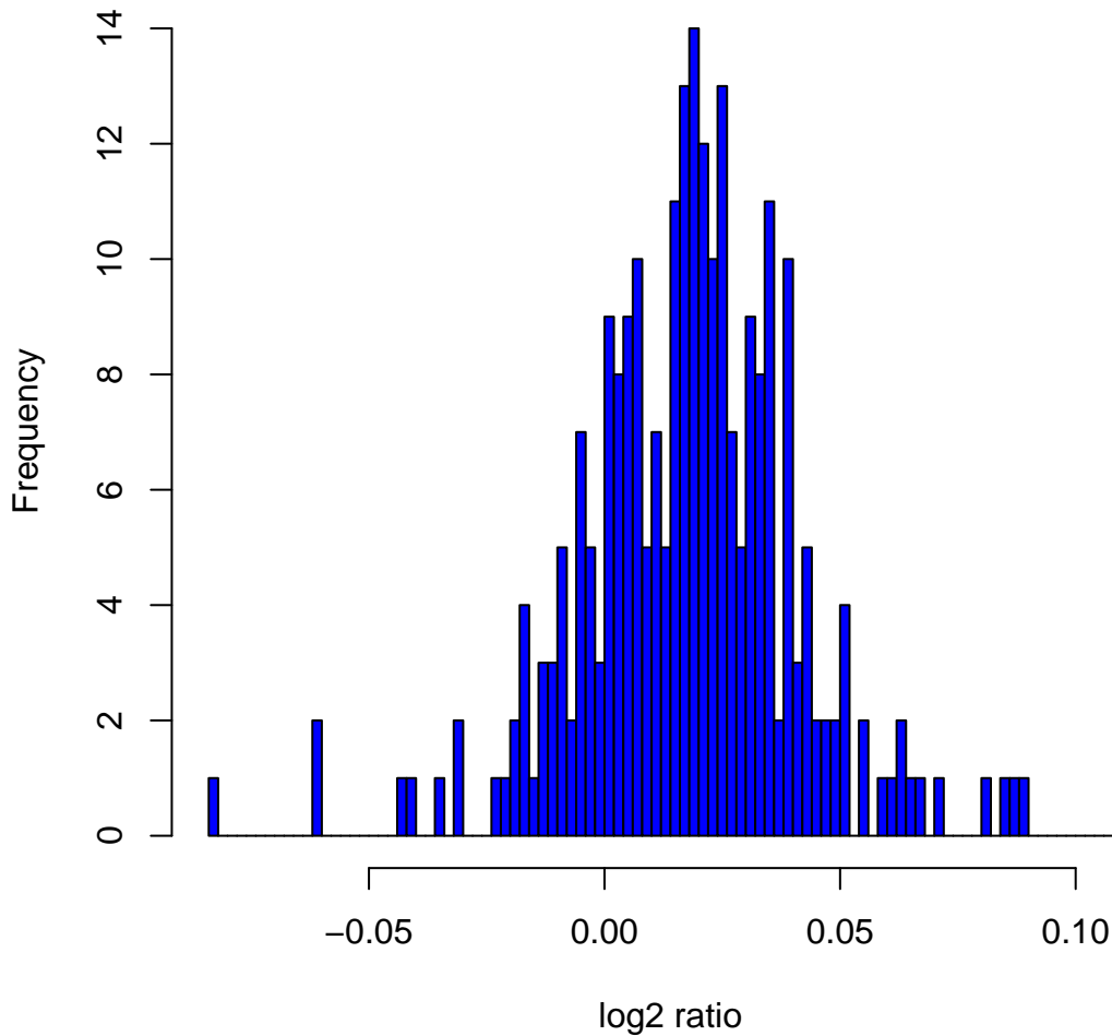
Histogram of log 2 ratios in 270 HapMap samples at clone Chr5tp-9E5
