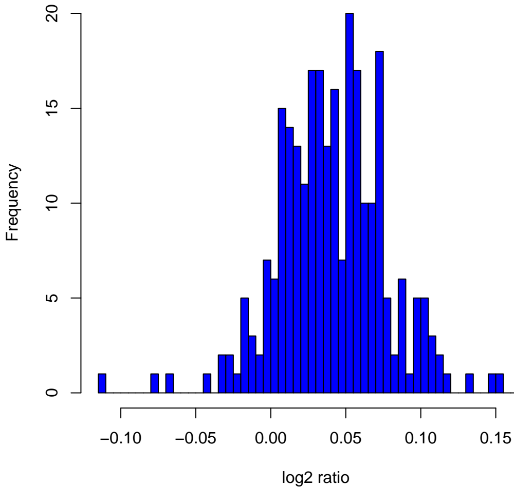
Histogram of log 2 ratios in 270 HapMap samples at clone Chr5tp-9H6
