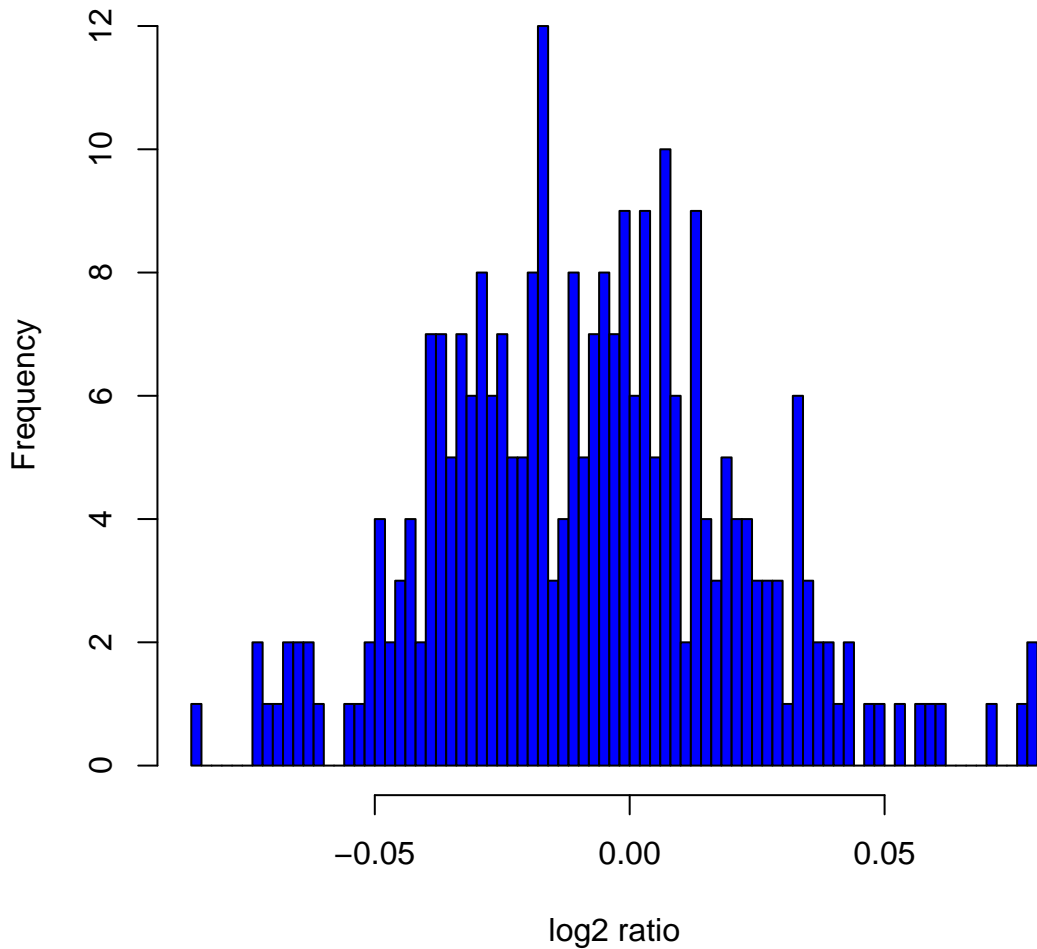
Histogram of log2ratios in 270 HapMap samples at clone Chr6tp-10B11
