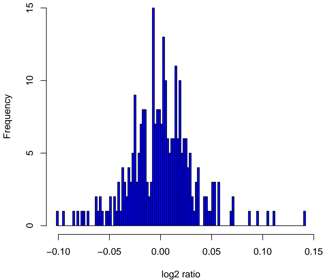
Histogram of log 2 ratios in 270 HapMap samples at clone Chr6tp-10B9
