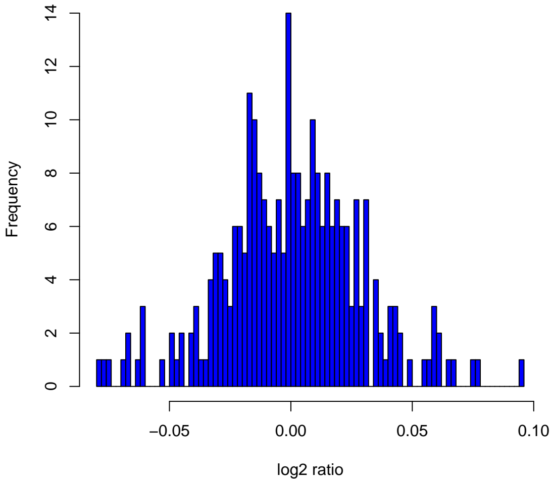
Histogram of log2ratios in 270 HapMap samples at clone Chr6tp-10C10
