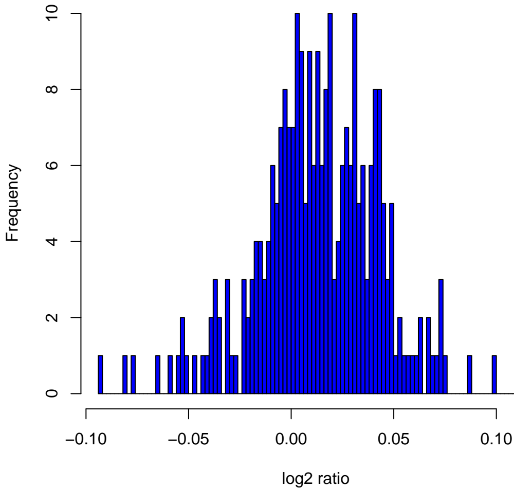
Histogram of log 2 ratios in 270 HapMap samples at clone Chr6tp-10D2
