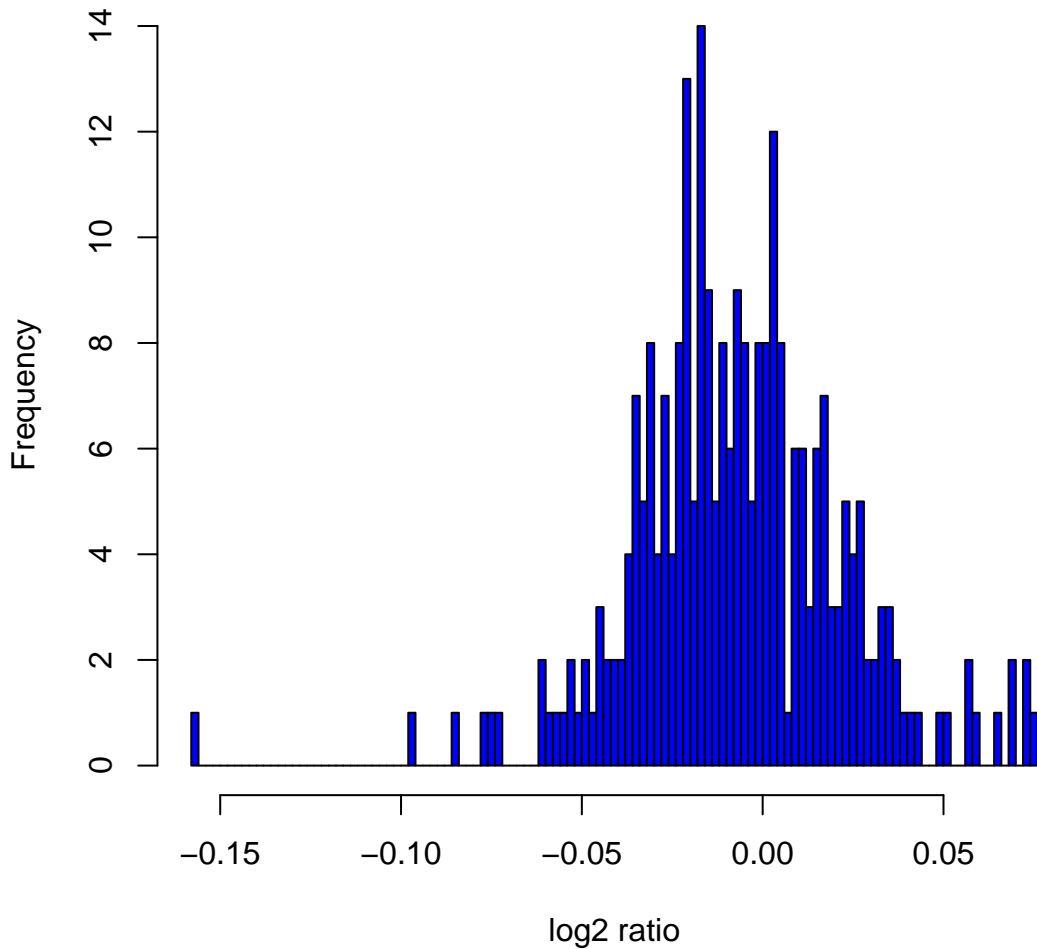
Histogram of log 2 ratios in 270 HapMap samples at clone Chr6tp-10E6
