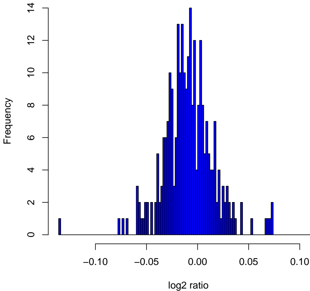
Histogram of log 2 ratios in 270 HapMap samples at clone Chr6tp-10G2
