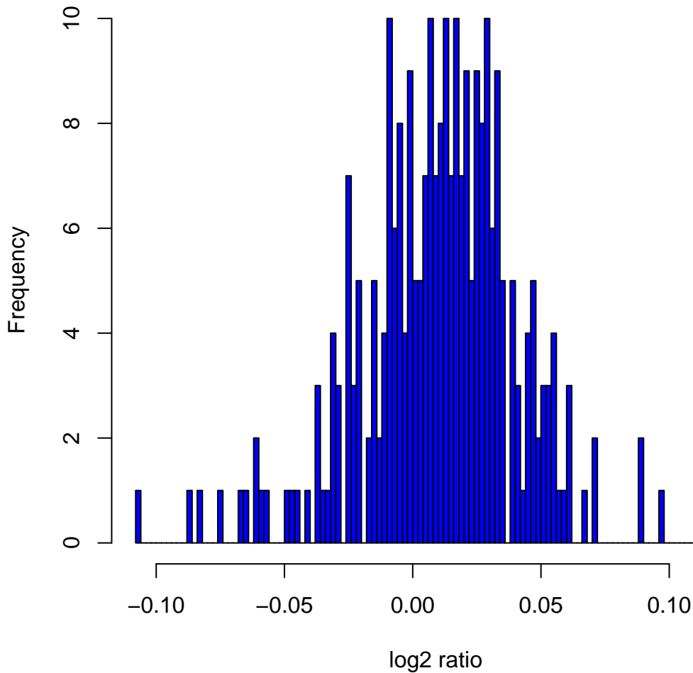
Histogram of log 2 ratios in 270 HapMap samples at clone Chr6tp-10H3
