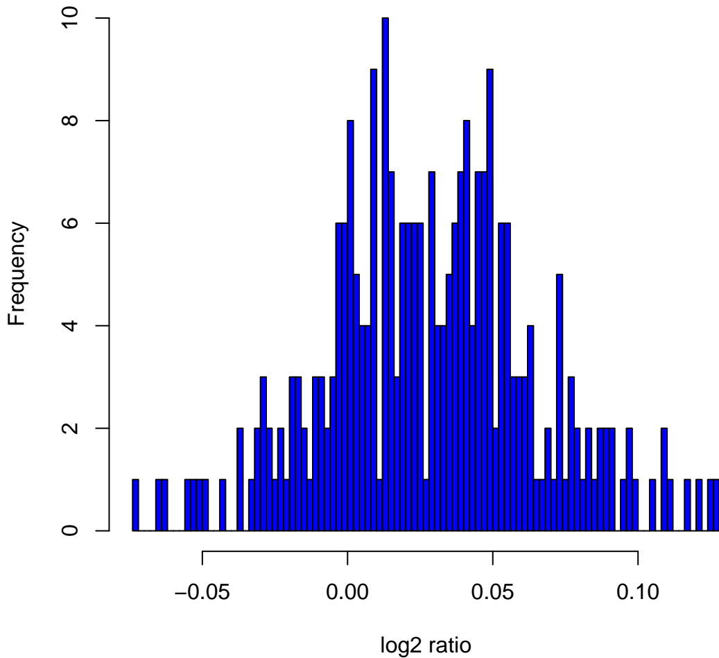
Histogram of log 2 ratios in 270 HapMap samples at clone Chr6tp-10H9
