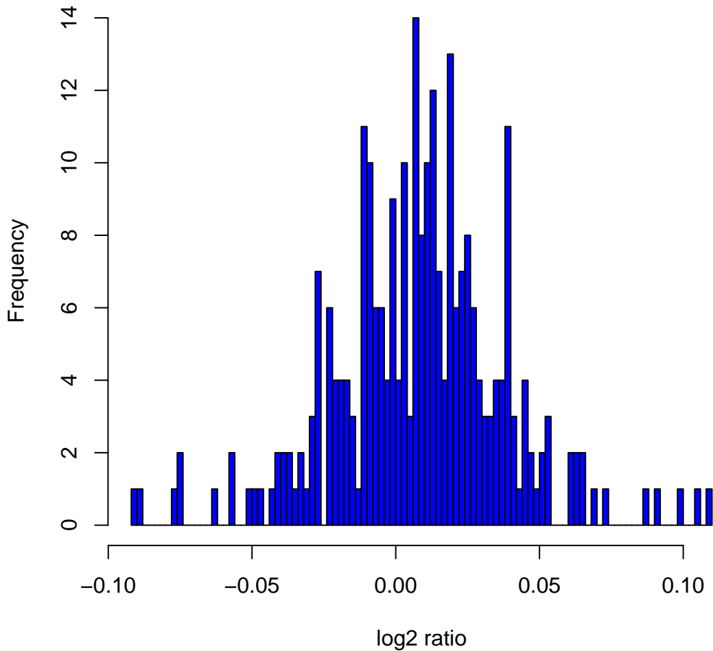
Histogram of log 2 ratios in 270 HapMap samples at clone Chr6tp-11C4
