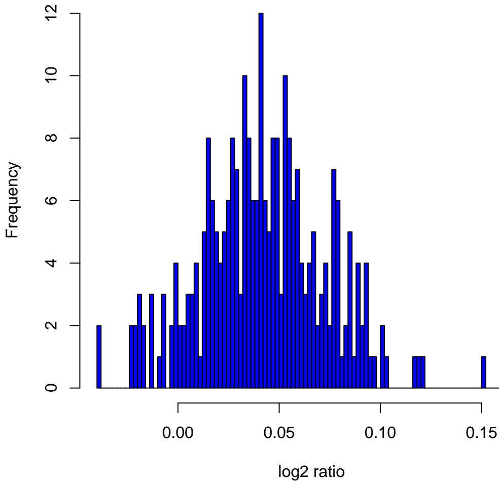
Histogram of log2ratios in 270 HapMap samples at clone Chr6tp-11C6
