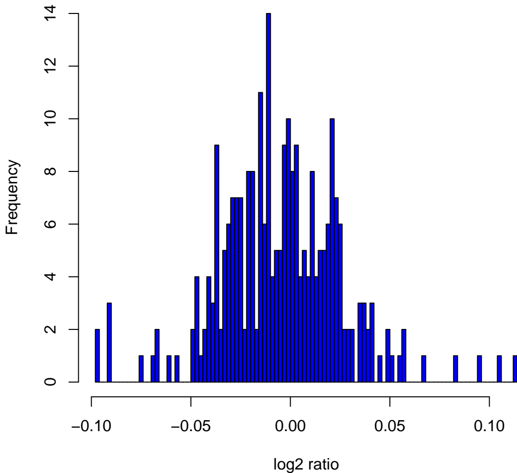
Histogram of log 2 ratios in 270 HapMap samples at clone Chr6tp-11C9
