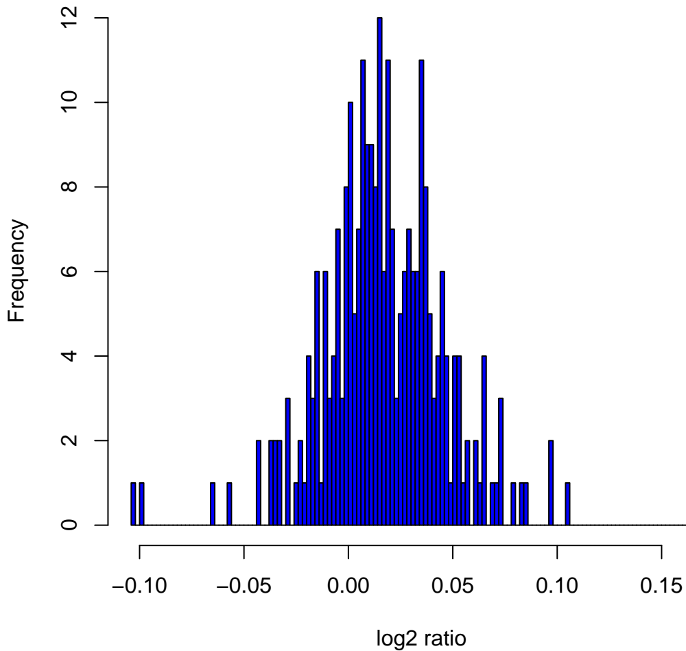
Histogram of log2ratios in 270 HapMap samples at clone Chr6tp-11D10
