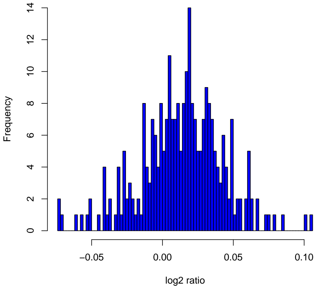
Histogram of log 2 ratios in 270 HapMap samples at clone Chr6tp-12A9
