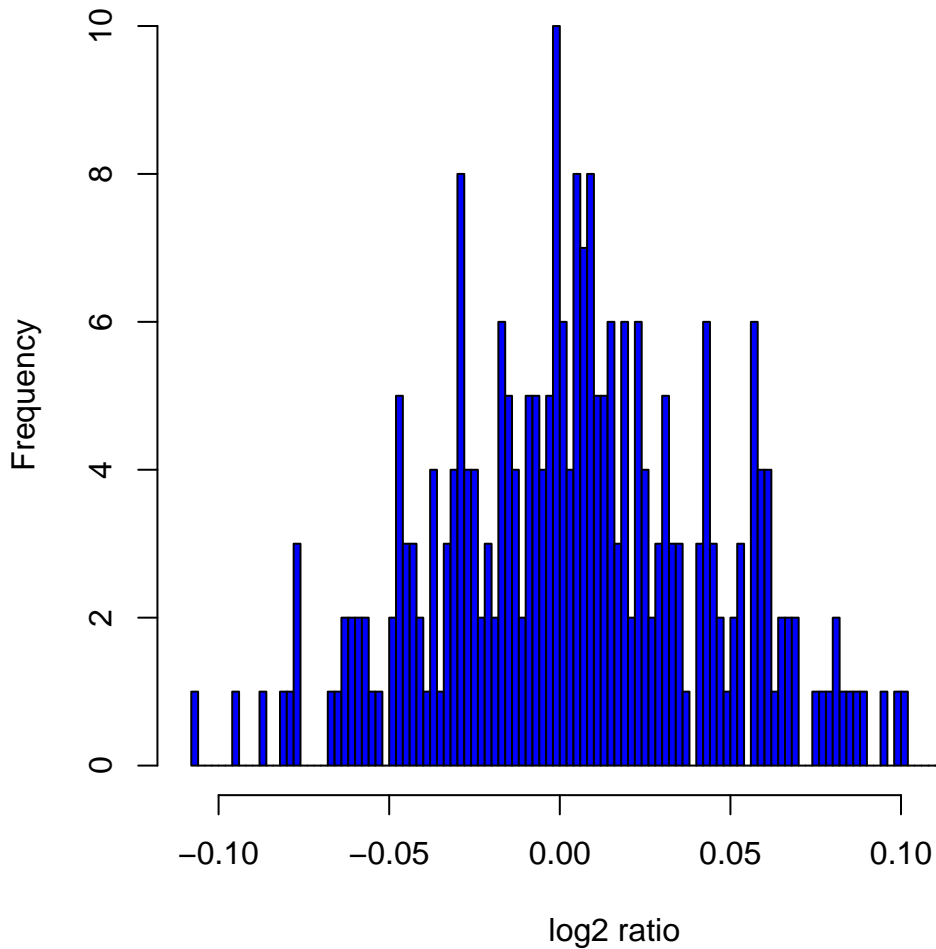
Histogram of log 2 ratios in 270 HapMap samples at clone Chr6tp-12B9
