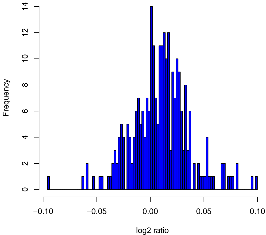
Histogram of log 2 ratios in 270 HapMap samples at clone Chr6tp-12G4
