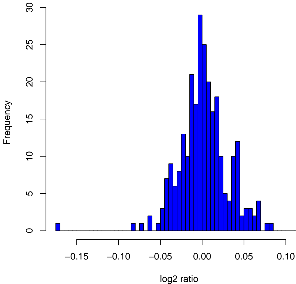
Histogram of log 2 ratios in 270 HapMap samples at clone Chr6tp-13B9
