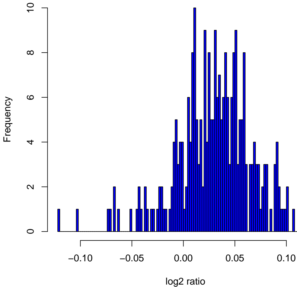
Histogram of log 2 ratios in 270 HapMap samples at clone Chr6tp-13E5
