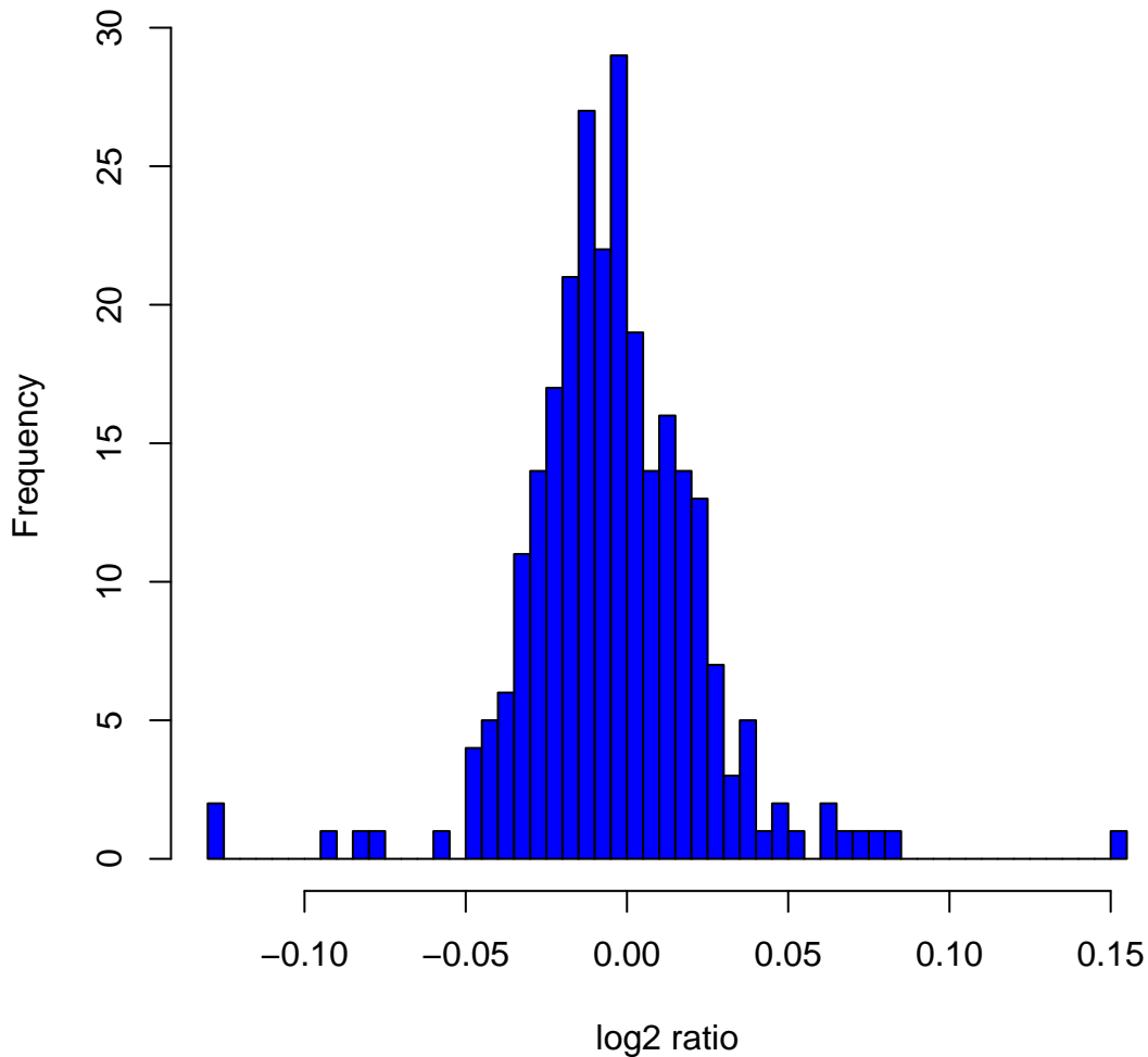
Histogram of log2ratios in 270 HapMap samples at clone Chr6tp-13F12
