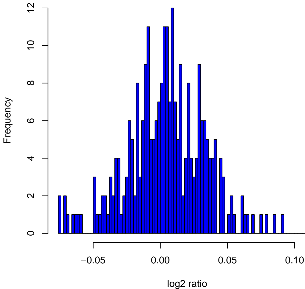
Histogram of log 2 ratios in 270 HapMap samples at clone Chr6tp-13G7
