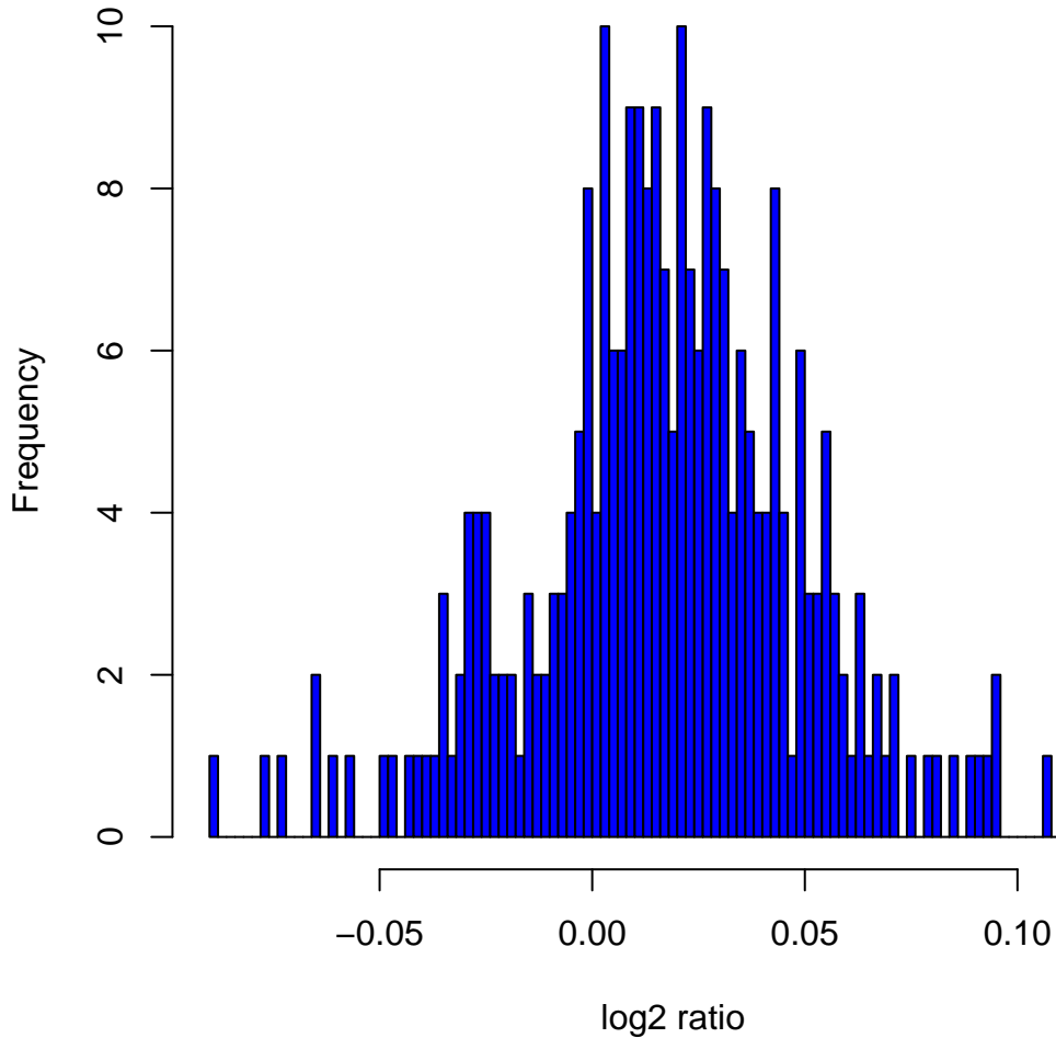
Histogram of log 2 ratios in 270 HapMap samples at clone Chr6tp-14B3
