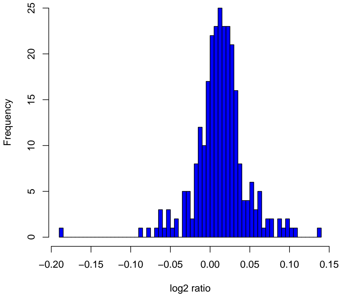
Histogram of log2ratios in 270 HapMap samples at clone Chr6tp-14C10
